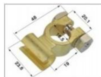
DJQ93082-35 2 负极
